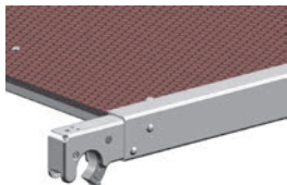
1241.190 Staro-Belagbrücke 1,9 m
