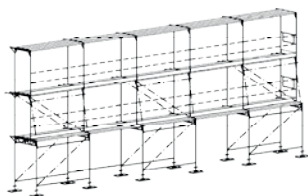
3D - Skizze
